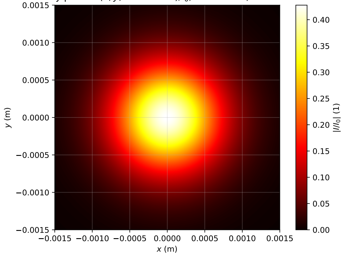
Intensity profile I(x, y, z = 3.742m)/I_0 , P_{in}=0.5P_{cr} , artificial time
